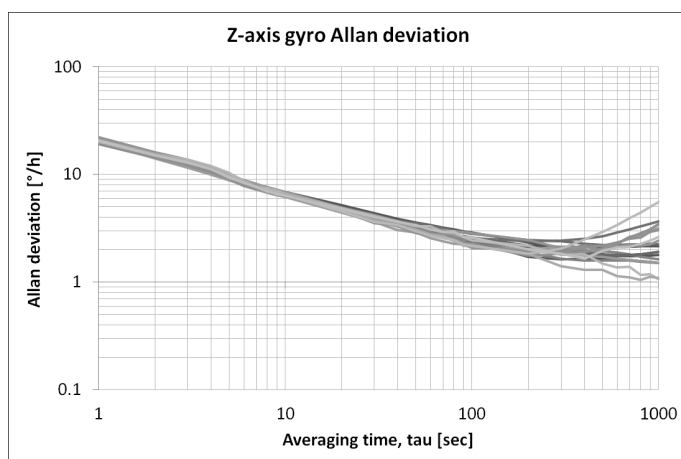
Figure 5. SCC2230-E02 gyro typical Allan deviation in ^{\circ}/h .
