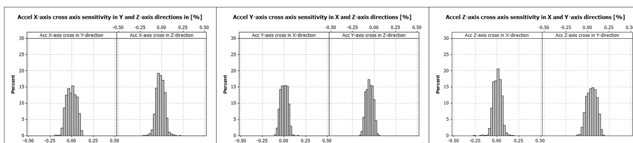
Figure 12. SCC2230-E02 accelerometer typical cross axis sensitivity in %.
