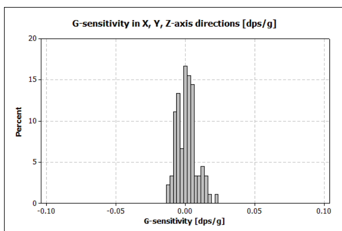
Figure 7. SCC2230-E02 gyro typical G-sensitivity in (^{\circ}/s)/g .
